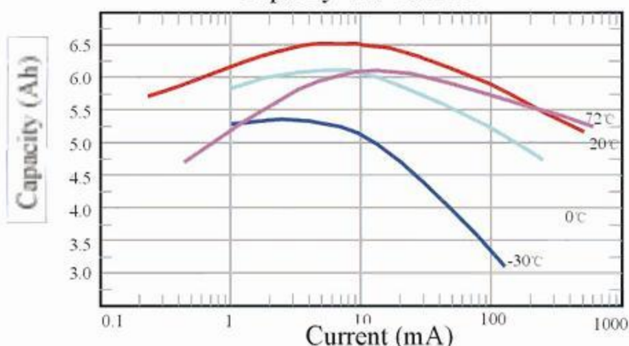
Capacity VS. Current
