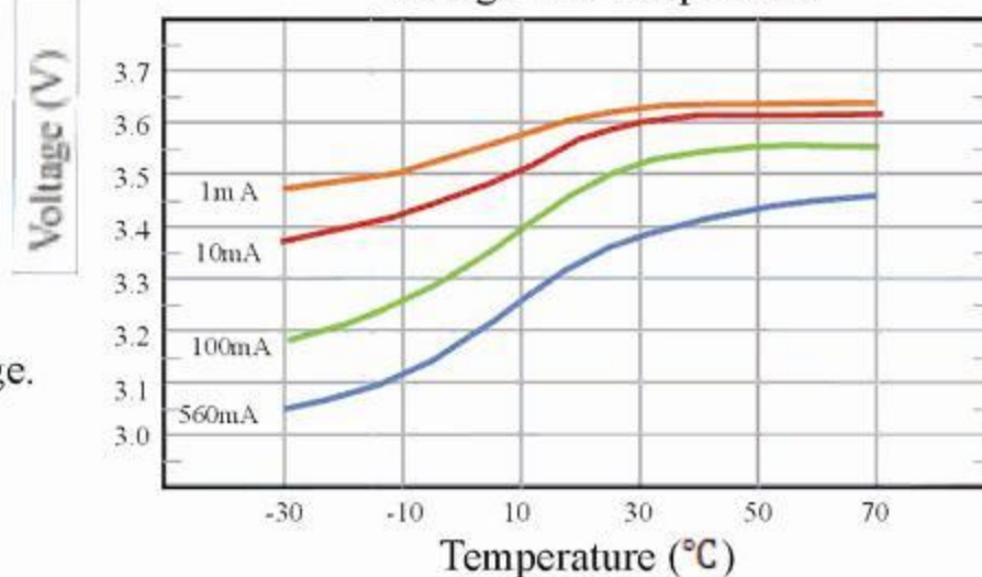
Voltage VS. Temperature
