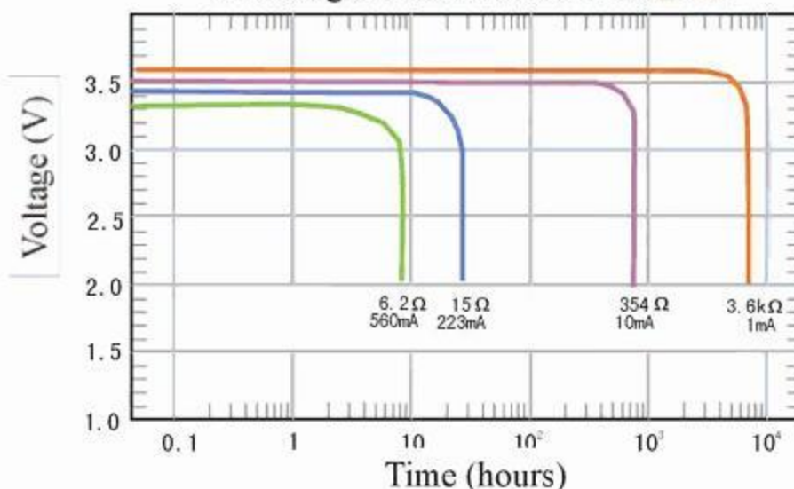
Discharge Characteristics at 23±2°C
